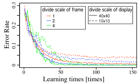
図 5: Error rate of experiment
