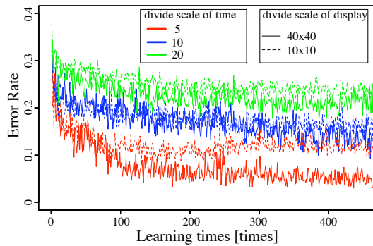
図 11: Error rate of experiment with attention module
