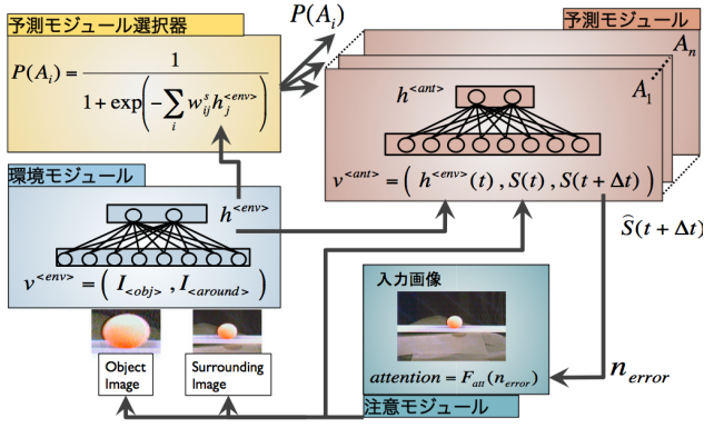
図 1: Model of situation-dependent predictor
